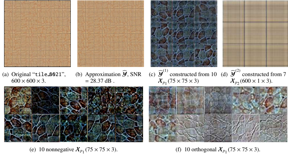
Fig. 1. Illustration for orthogonal and nonnegative pattern decompositions of the image "tile_0021". (b)-(d) reconstructed images and two basis images by 10 patterns of size 75 \times 75 \times 3 and 7 patterns of size 600 \times 1 \times 3 . (e)-(f) 10 nonnegative and orthogonal patterns.
