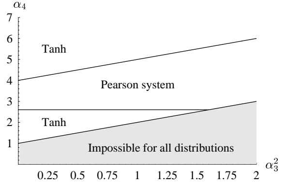
Figure 2: The contrast functions used in the Pearson-ICA are presented in (\alpha_3^2, \alpha_4) -plane. Limit for all distributions is line \alpha_4 = \alpha_3^2 + 1 . Clearly sub-gaussian sources are defined to have kurtosis less than 2.6 and the tanh-contrast is utilized. Clearly super-gaussian sources are defined to have \alpha_4 = \alpha_3^2 + 4 and the tanh-contrast is again utilized. In area between these boundaries the Pearson system is used. The choice of boundaries is based on practical experience.
